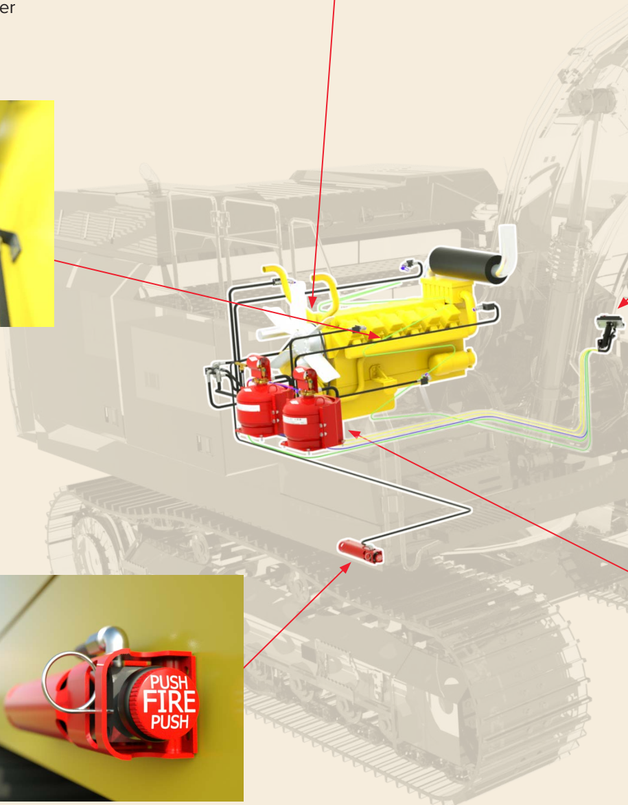
Engine Compartment
